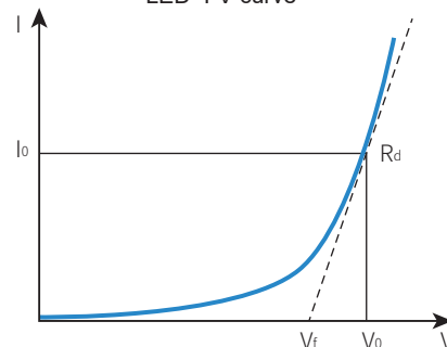
LED I-V curve
